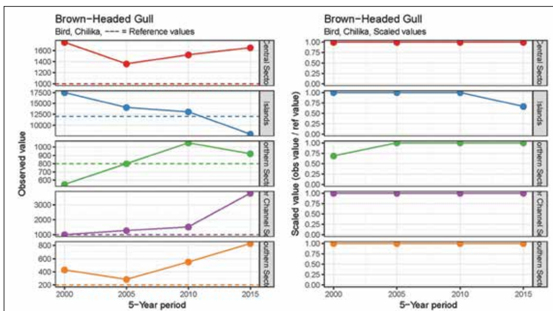
Figure 30: Observed and scaled value of Brown headed gull
